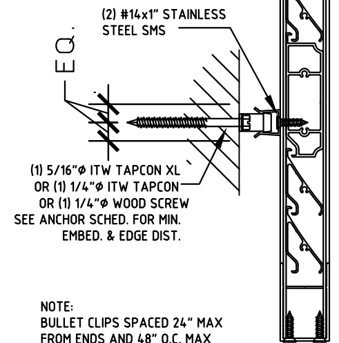
(X2) OPEN POSITION LOCK W/ BULLET CLIP SCALE: 3" = 1'-0"
