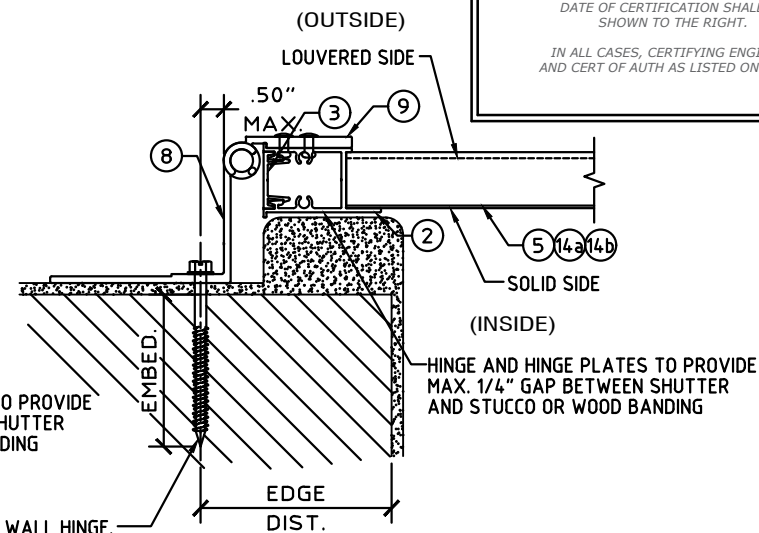
(N4) ALTERNATE WALL HINGE CONNECTION SCALE: 3" = 1'-0"
